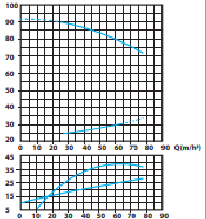
SEN 50-250A Pump Performance Curve
