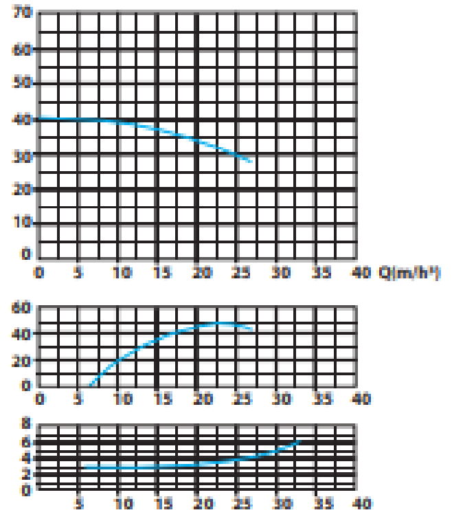
SEN 32-200C Pump Performance Curve
