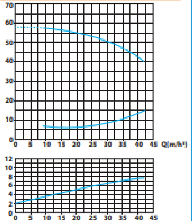
SEN 40-200A Pump Performance Curve
