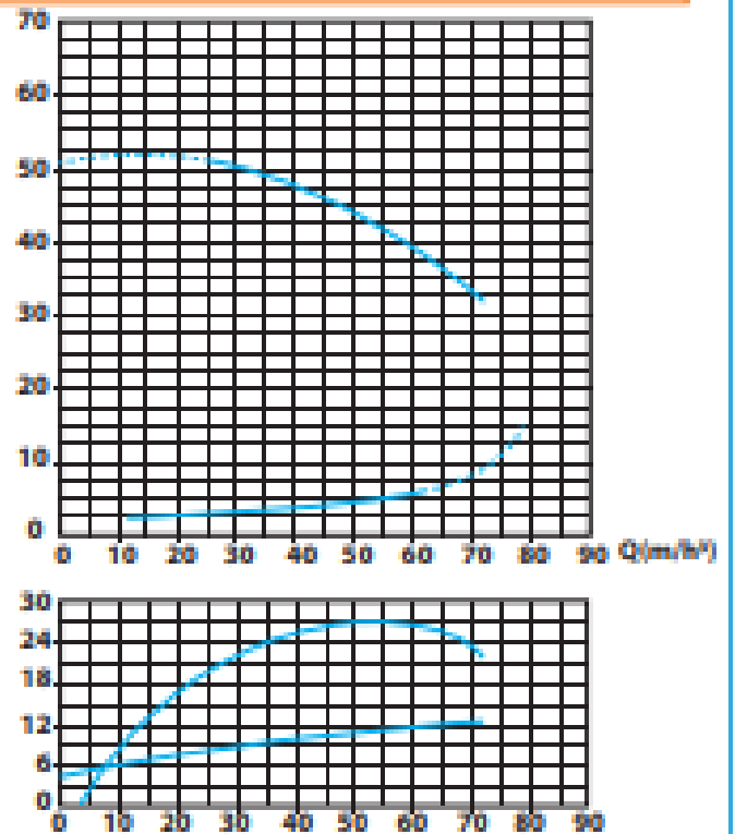
SEN 50-200B Pump Performance Curve
