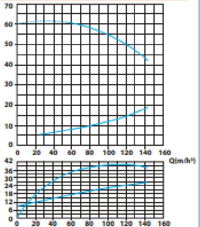
SEN 65-200A Pump Performance Curve
