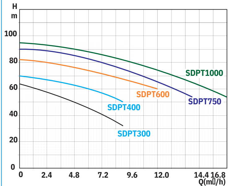
SDPT Pump Performance Curve
