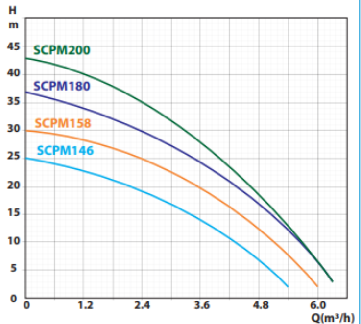
SCPM Pump Performance Curve
