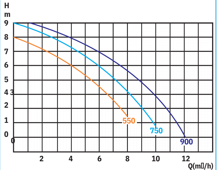
SPA Pump Performance Curve
