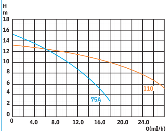
SWVS Pump Performance Curve
