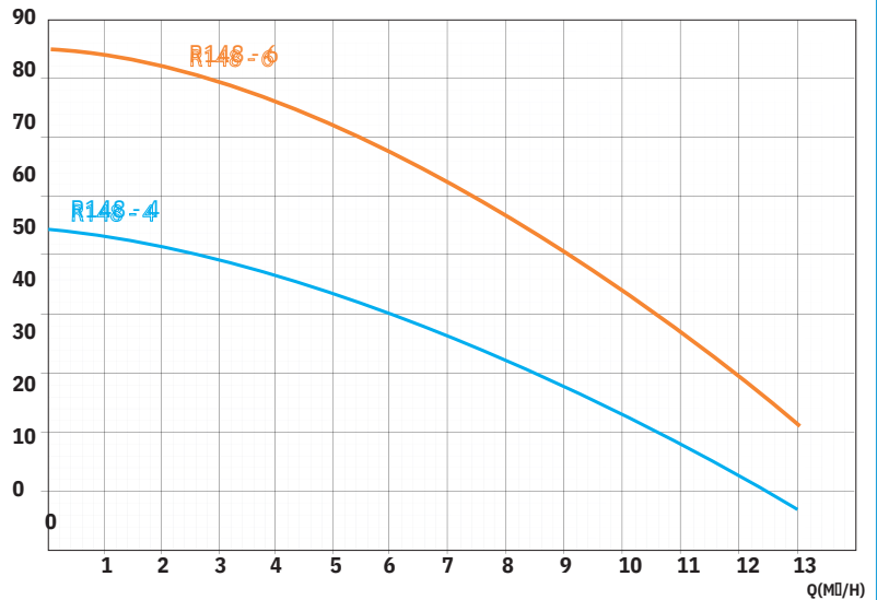
R128K Pump Performance Curve
