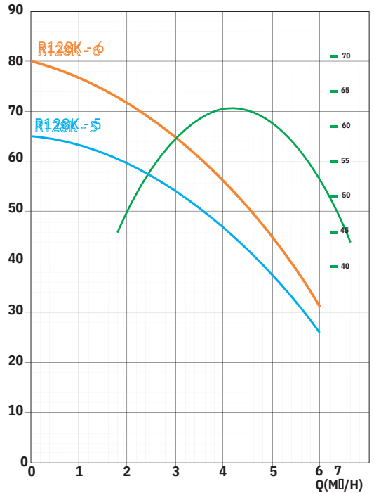
R128K Pump Performance Curve
