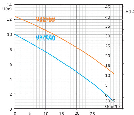
MSC Pump Performance Curve
