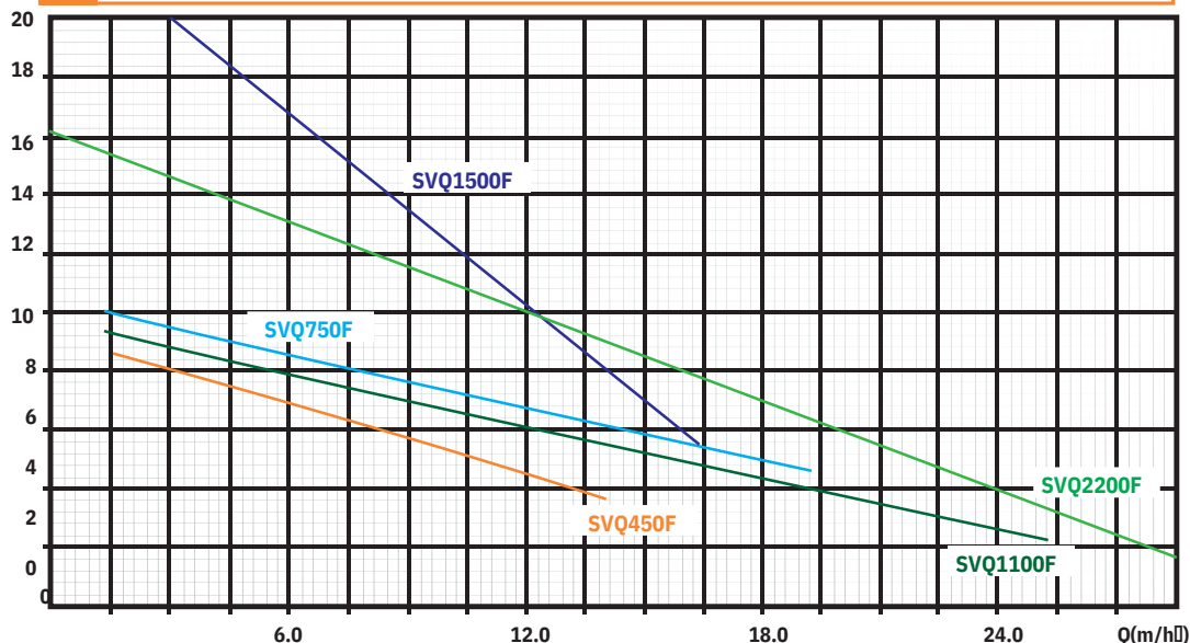
SVQ Pump Performance Curve
